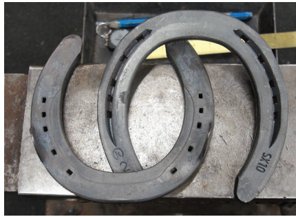
SX-10 fronts have sole relief built-in and the thickness of the shoe allows you to add even more if needed. Clipped fronts have solid clips between the second and third nail hole.
